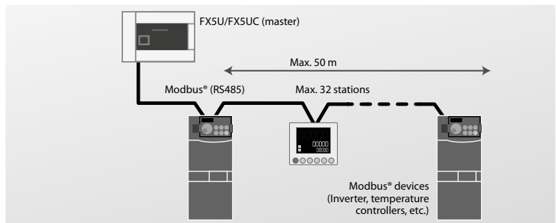
Modbus® communication
