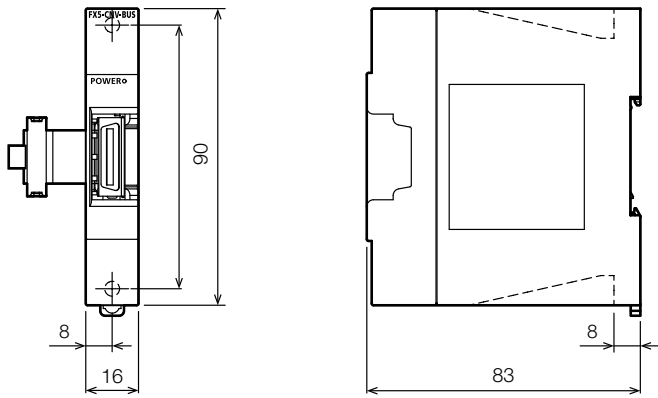
FX5-CNV-BUS
