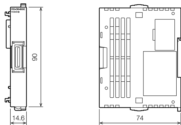
FX5-CNV-BUSC
