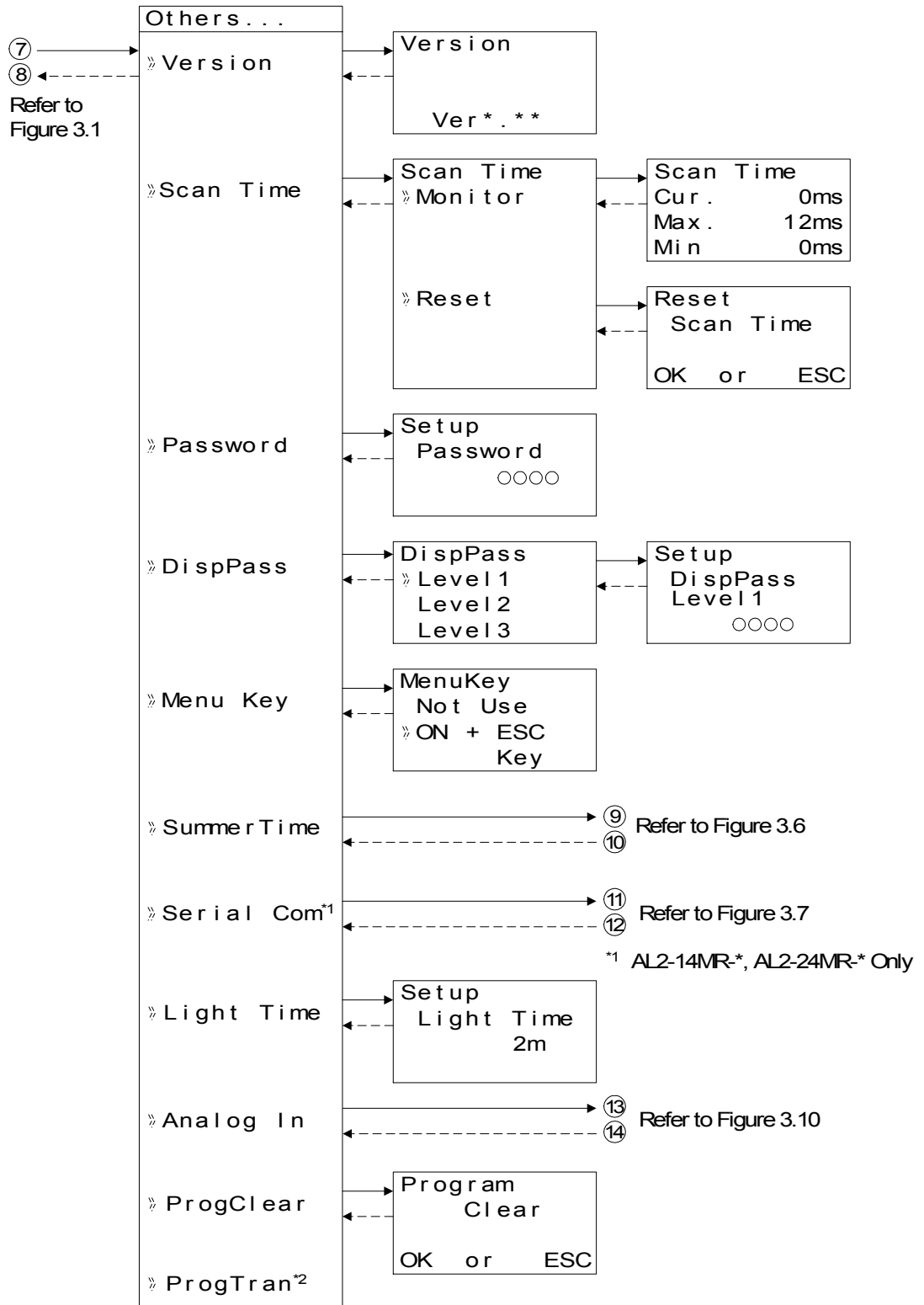
Figure 3.5: Others Menu in Stop Mode Operation
