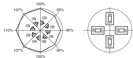
Fig.: Change of the rated current with mounting position deviating from the vertical
