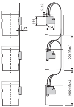
Vertical mounting
